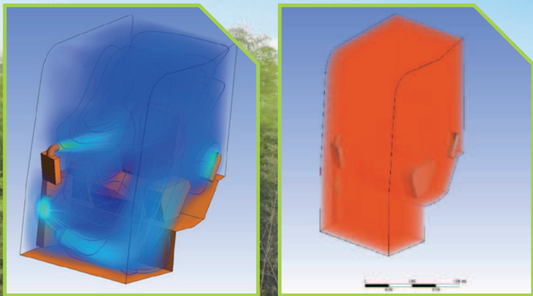
New air duct design, 8 air outlet, air outlet adjustment range, 360° flow field around the driver, good cooling effect. The large displacement compressor, with 46% more cooling capacity than the competition, enters the cab and is as cool as an autumn day.
