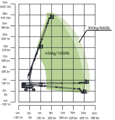
Range of Motion ZT88J
