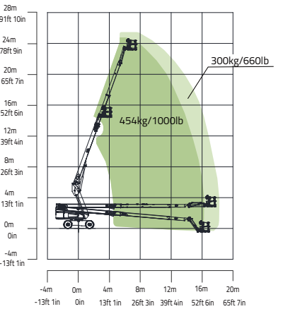
Range of Motion ZT76J
